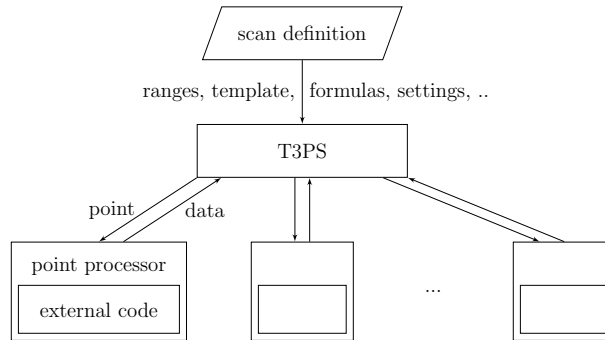
Figure 1: Flow chart representing the overall algorithmic structure of a scan in T3PS. The main program takes the information provided by the scan definition file and distributes the work to a certain number of concurrently running point processors , one point each. These in turn calculate data using some (possibly external) code and return the relevant data.
