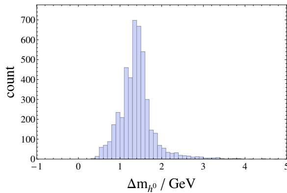
Figure 7: Difference between the Higgs mass as calculated by the codes softSUSY and SPheno for the points found in the “explorer” scan.
